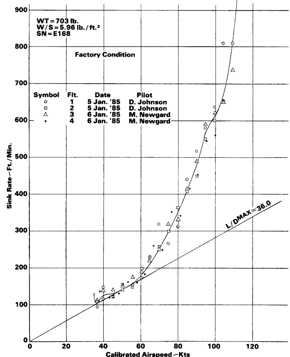
FIGURE 2 DG-101G N101TX POLAR TEST DATA
